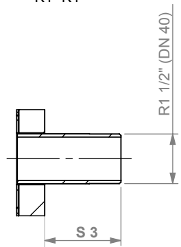
Anschluß / Connection / Raccordements K1 - K4
